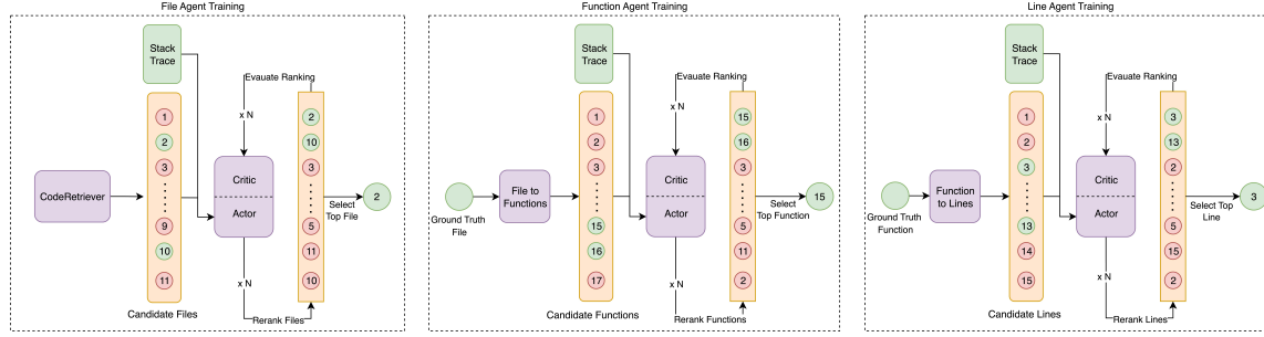
Fig. 4. C2C hierarchical training pipeline. The diagram shows the sequential training strategy (TWF), where agents are trained using ground-truth oracle inputs to ensure stability.
